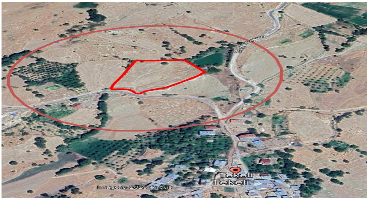
Figure 24. Area of Influence of Plot No. 155/30 in Tekeli Village
