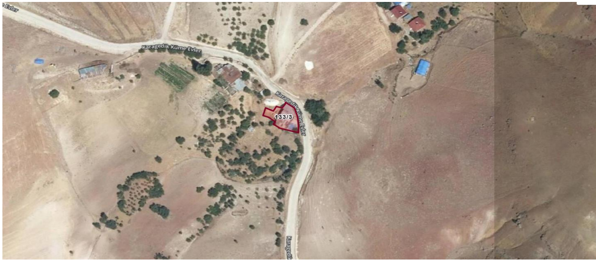
Figure 25. Satellite Image of Plot No. 133/3 in Toratlı Village
