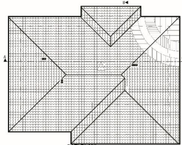
ÇATI PLANI
