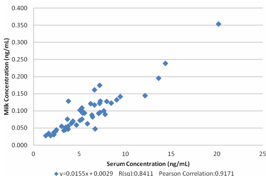
Figure 4.2.4: PFOS concentrations (ng/mL) in serum and milk samples from Sweden, 2004-2011. The linear equation of the line, including R^2 , is given together with Pearson's correlation coefficient.
