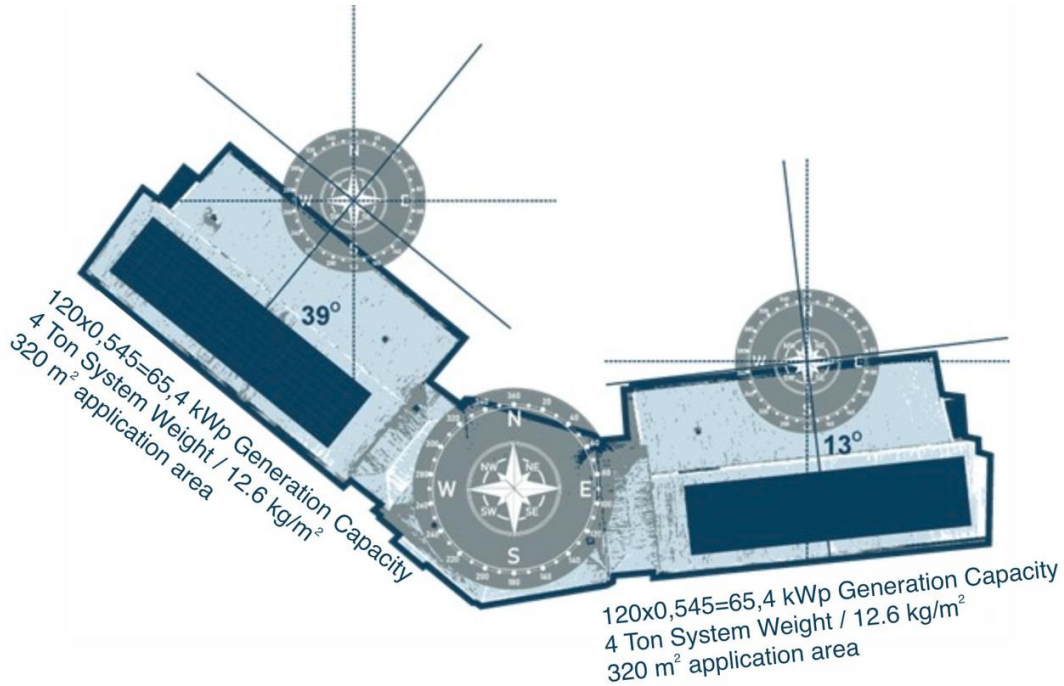
Figure 9 Kocaeli- Ministry Of Youth And Sports Kandira Special Provincial Administration Kyk Dormitory Building Roof Top PV Layout Plan
