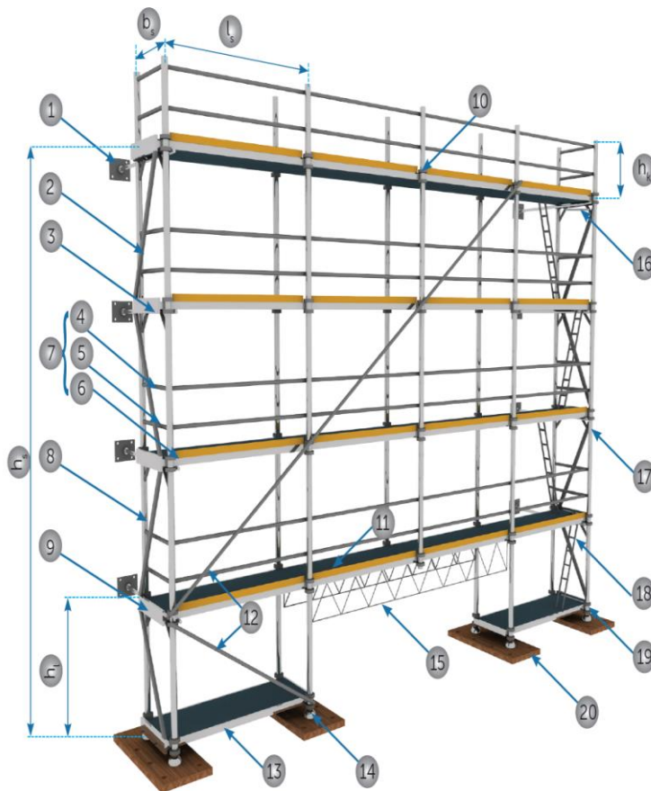
Figure 9: Exterior Scaffolding Sample Image
